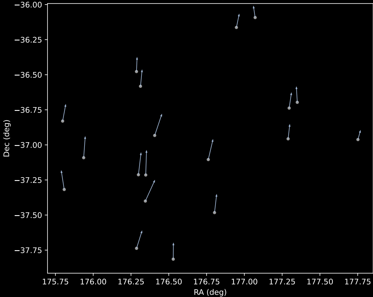
GALAH DR4 Cluster 1 Proper Motion Vectors (n=19)
