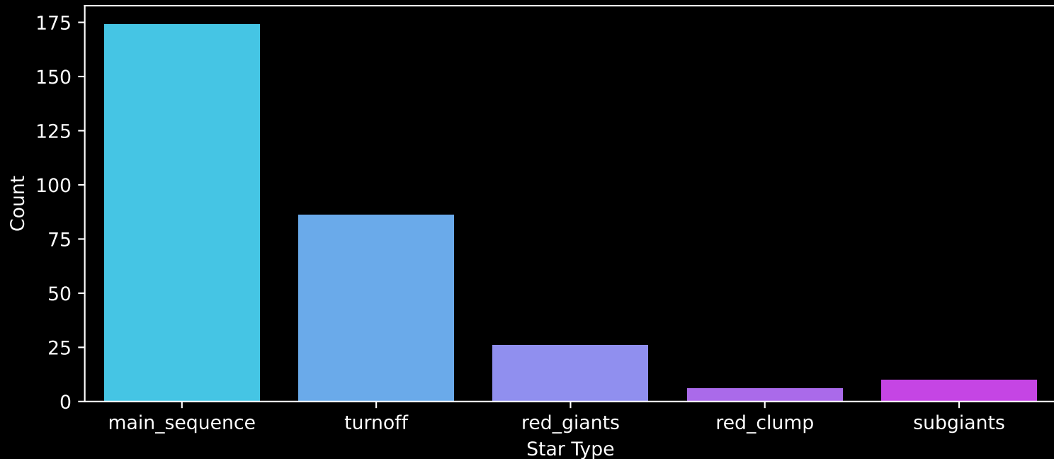
GALAH DR4 Field: [481] Count plot of Star Type
