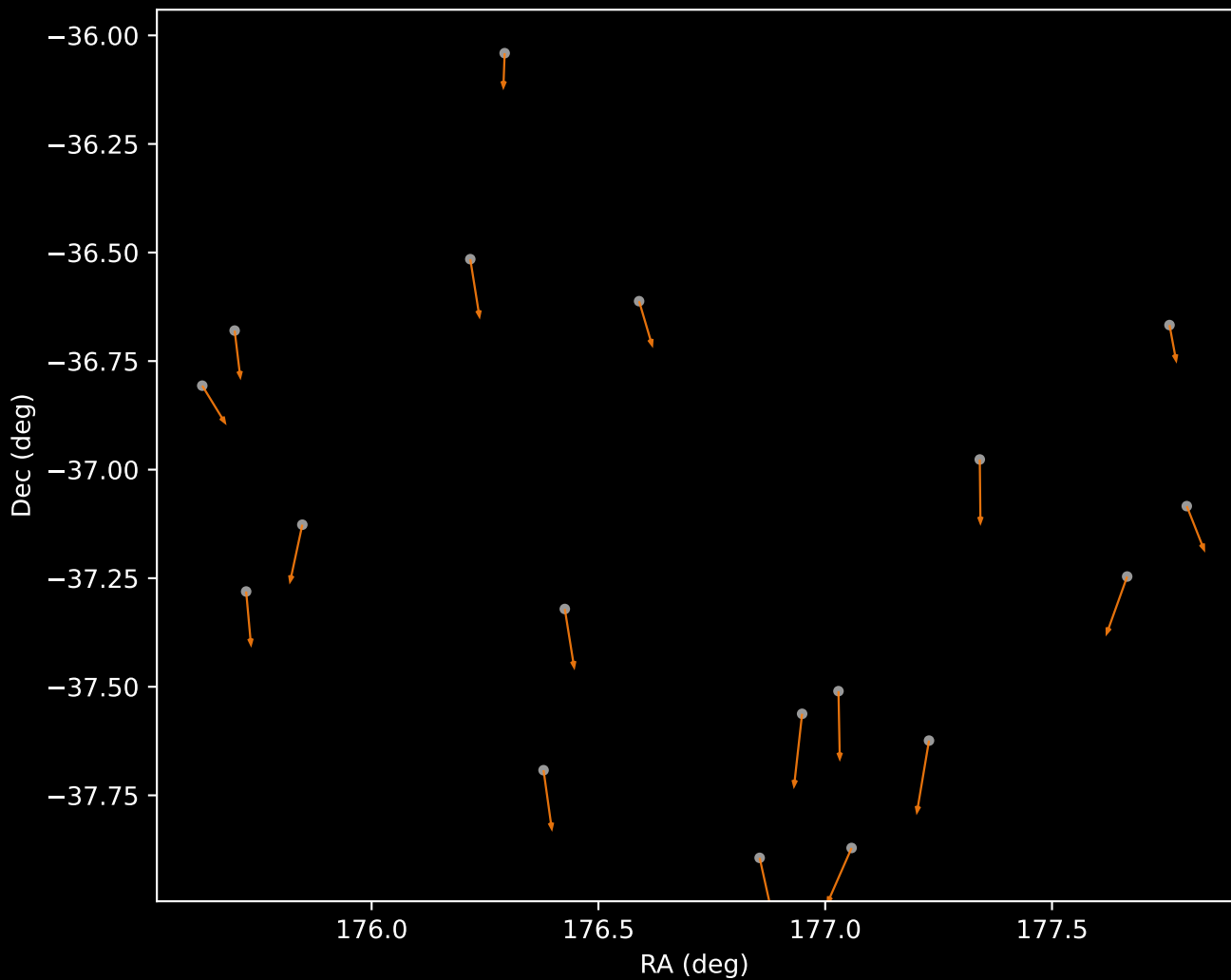
GALAH DR4 Cluster 2 Proper Motion Vectors (n=18)
