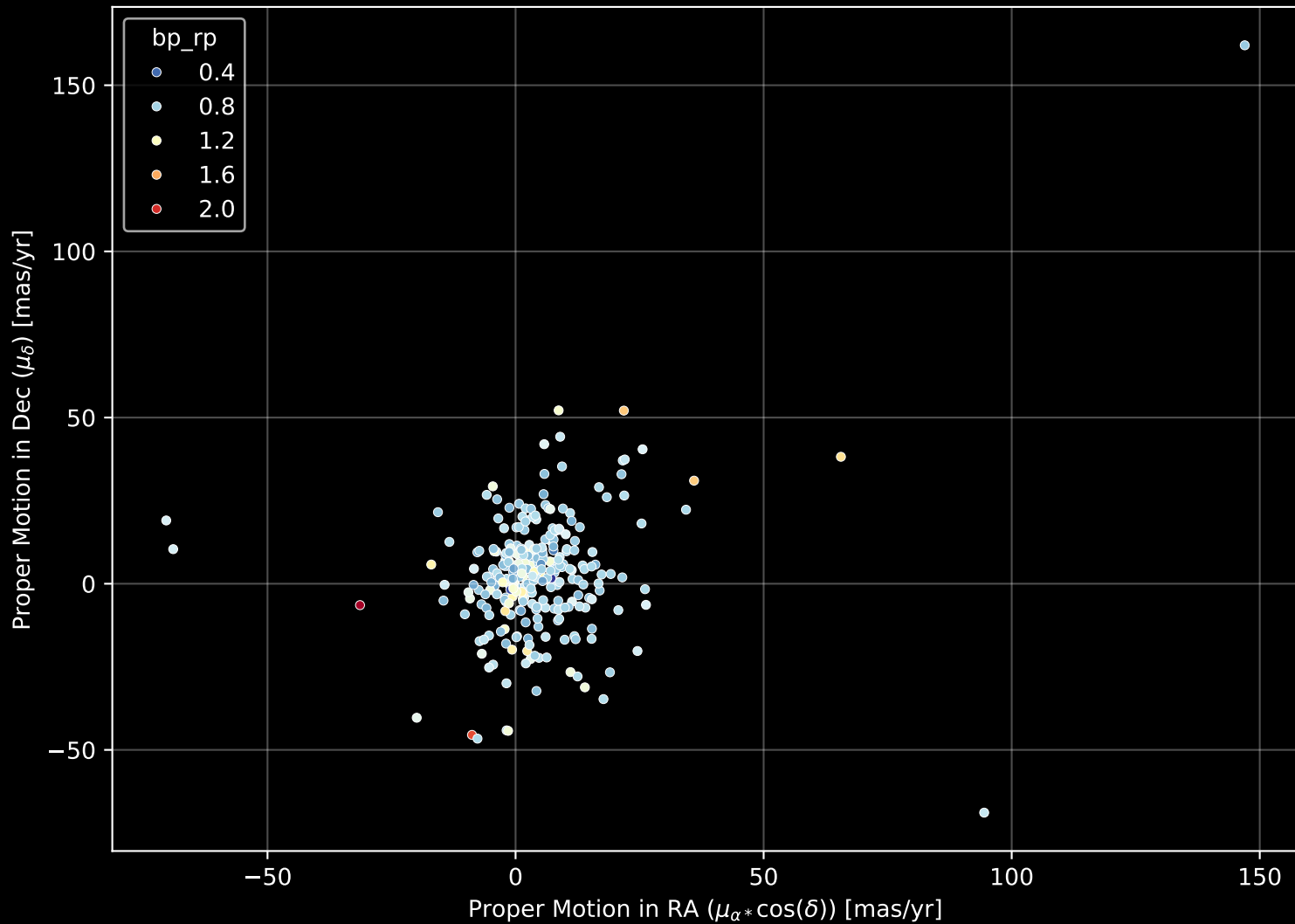
GALAH DR4 Field: [481] Proper Motion Diagram (n= 302)
