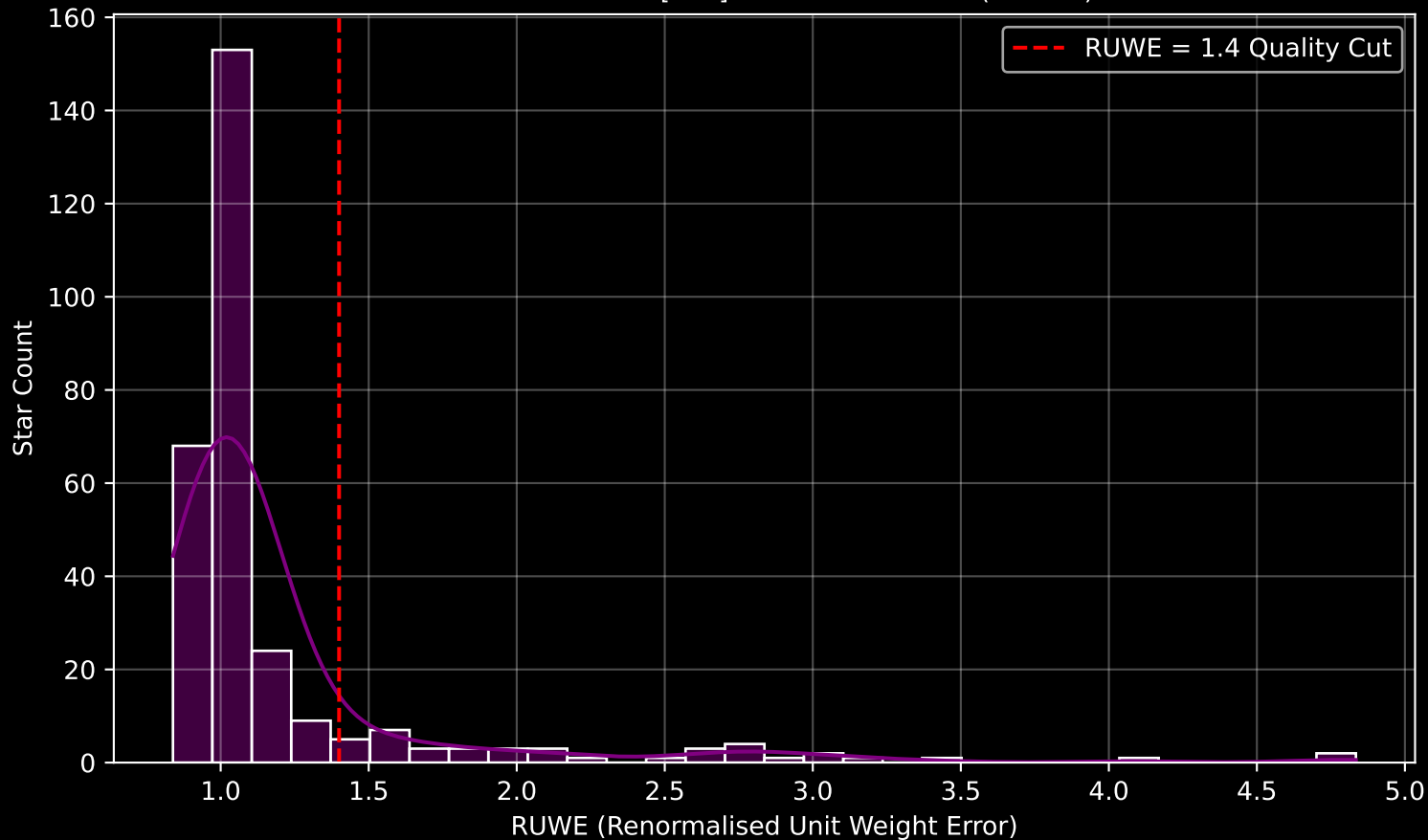
GALAH DR4 Field [481] RUWE Distribution (n= 295)
